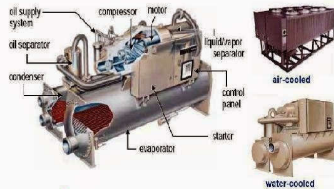
Screw
